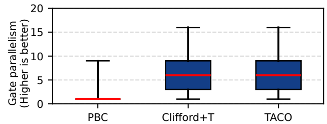
Fig. 14. Gate parallelism comparison of 20-qubit QFT. TACO preserves the same high gate-level parallelism as the original Clifford+T circuit.
