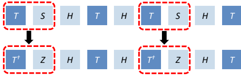
Fig. 7. Remove Phase ( S ) gate using the identity: TS = T^\dagger Z .
