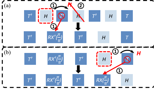
Fig. 9. Commuting all the Hadamard gates to the end of the sequence using the commuting rules in Equation 7. Circled numbers indicate the step order.
