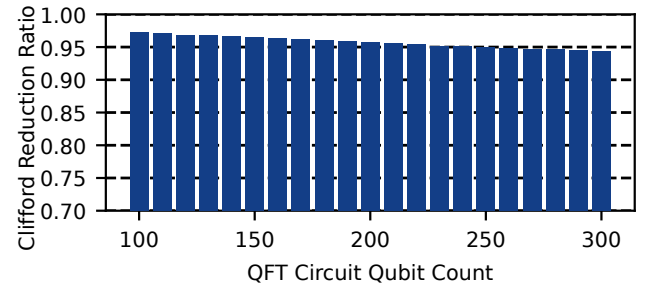
Fig. 20. Clifford gate reduction ratios achieved by TACO on QFT circuits ranging from 100 to 300 qubits. The reduction ratio remains consistently around 95% across all circuit sizes, demonstrating the scalability of TACO to large-scale fault-tolerant quantum circuits.
