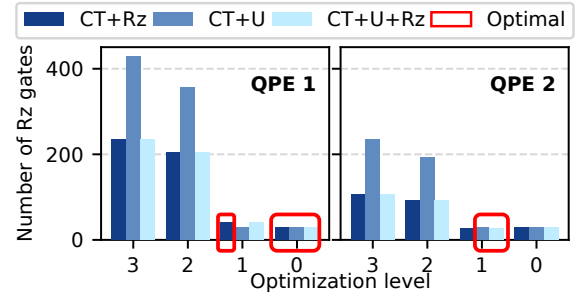
Fig. 11. Number of R_z gates in intermediate circuits obtained from transpiling two 4-qubit QPE circuits using Qiskit Transpiler across optimization levels 0-3 and three basis gate sets (Clifford+T+U, Clifford+T+Rz, Clifford+T+U+Rz). Lower R_z gate counts indicate better optimization.
