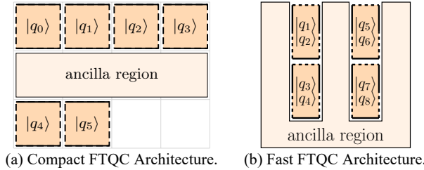
Fig. 19. PBC architectures for comparison.
