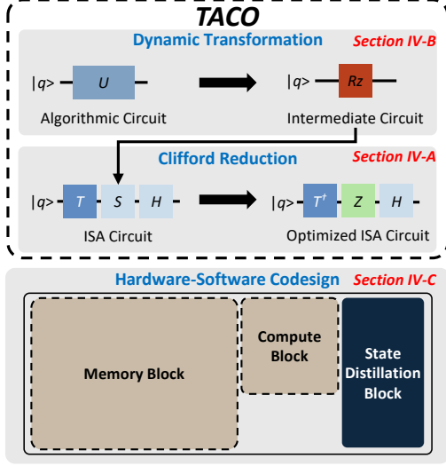
Fig. 6. Overview of the design. TACO begins with dynamic gate decomposition of the algorithmic circuit, transforming it into an intermediate form with reduced R_z gates before synthesizing into a Clifford+T circuit. TACO then applies Clifford reduction to minimize execution time. The resulting circuit's high locality of \pi/4 rotations informs a software-guided hardware design.
